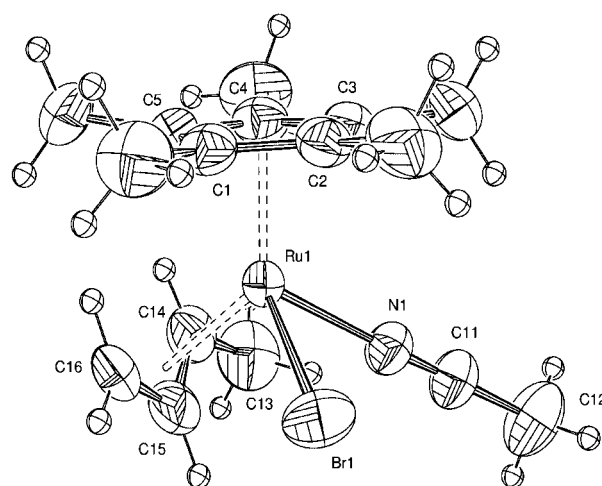
Figure 1. ORTEP drawing of 2d showing 50% thermal ellipsoids; selected bond distances (Å) and angles (°): Ru(1)–Br(1) 2.552(6), Ru(1)–N(1) 2.077(4), Ru(1)–C(14) 2.280(5), Ru(1)–C(15) 2.165(5), Ru(1)–C(16) 2.208(4), C(13)–C(14) 1.495(8), C(14)–C(15) 1.403(8), C(15)–C(16) 1.394(7), Br(1)–Ru(1)–N(1) 82.2(1), Br(1)–Ru(1)–C(16) 81.7(2), N(1)–Ru(1)–C(14) 82.7(2), C(13)–C(14)–C(15) 123.5(5), C(14)–C(15)–C(16) 115.8(5); the PF 6 anion and the water molecule are omitted for clarity.
