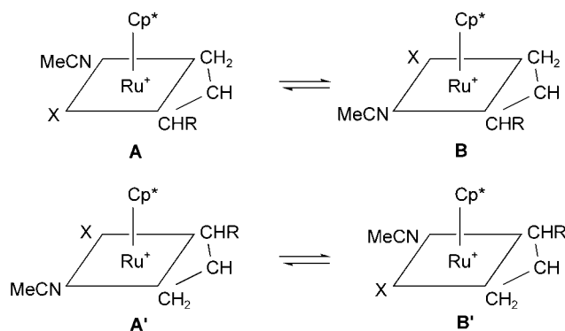
Scheme 2. Simple representation of the two stereoisomers of 2c–f as their enantiomeric pairs AA' and BB' (the formation of 2c–f is diastereoselective with respect to the chiral CHR and CH carbon atoms).
