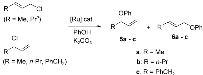
Scheme 4. Ruthenium-catalyzed synthesis of allyl phenyl ethers from aliphatic allylic chlorides.
