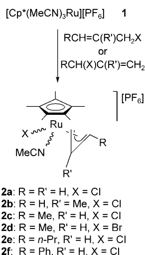
Scheme 1. Synthesis of the new complexes 2a–f .
