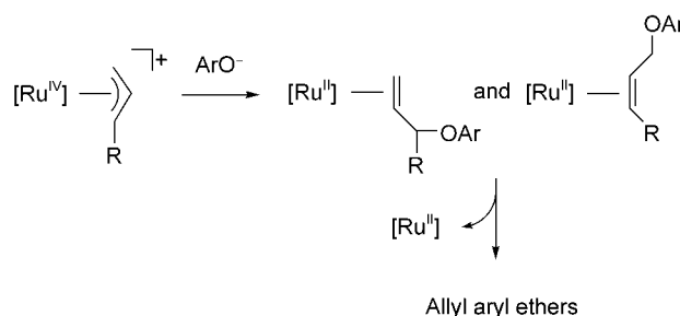
Scheme 5. A plausible mechanism for the ruthenium-catalyzed formation of allyl aryl ethers.
