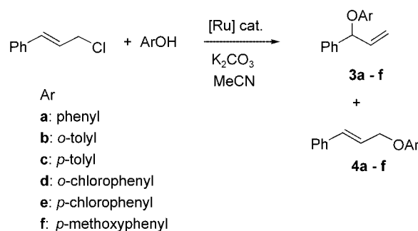
Scheme 3. Ruthenium-catalyzed synthesis of allyl aryl ethers from cinnamyl chloride.
